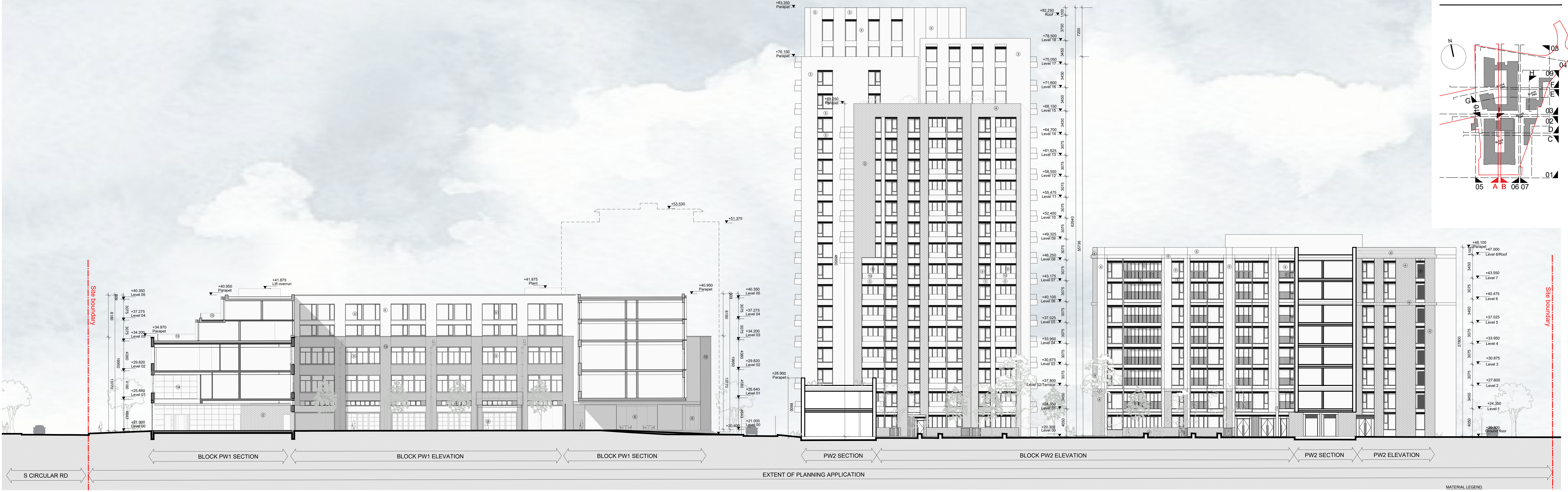
01 Section A Player Wills Site SCALE 1:200
